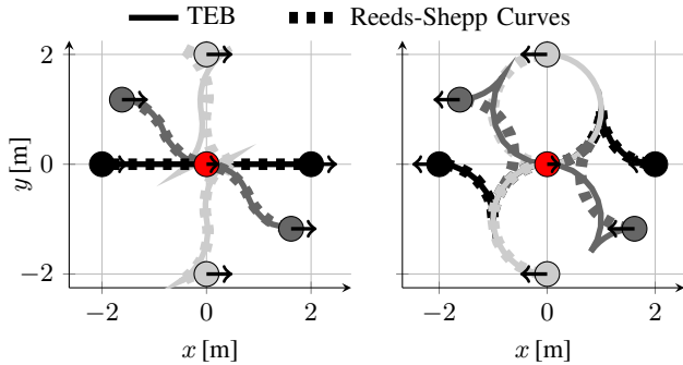
Fig. 2: TEB trajectories and RS curves for different goal configurations, left: \beta_f = 0 rad, right: \beta_f = \pi rad
